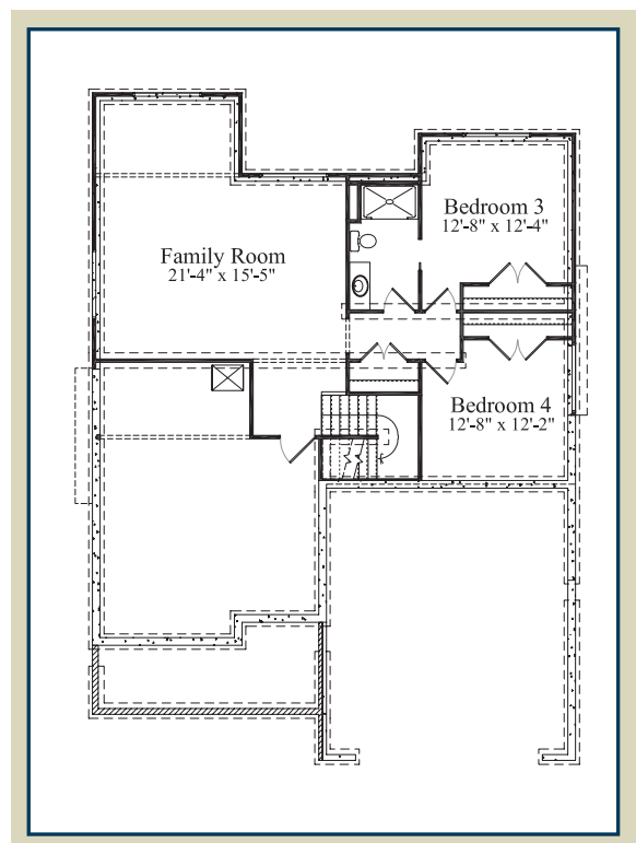
LOWER LEVEL RIGHT: 1030 SQ. FT.
