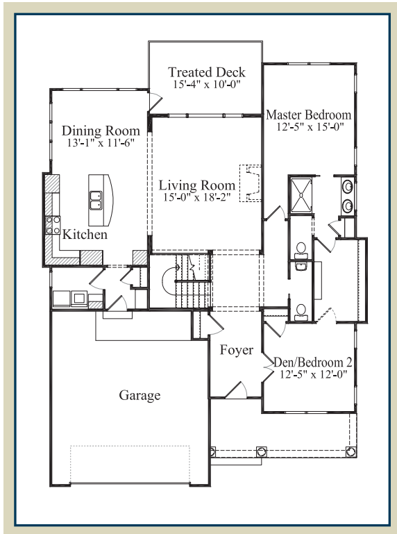
MAIN FLOOR LEFT: 1583 SQ. FT.
