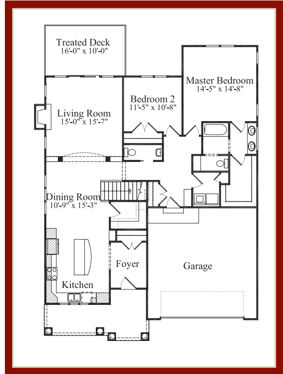
MAIN FLOOR RIGHT: 1546 SQ. FT.
