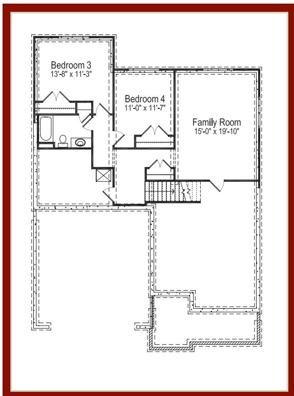
LOWER LEVEL LEFT: 917 SQ. FT.
